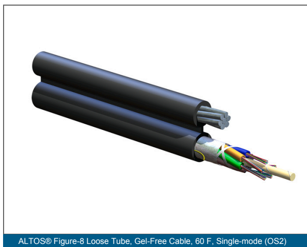
ALTOS® Figure-8 Loose Tube, Gel-Free Cable, 60 F, Single-mode (OS2)
